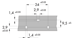
FORATURA SUGGERITA PER: TO220 HOLES LAYOUT FOR CASING: TO220
